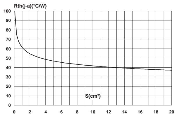
Fig. 10: Thermal resistance junction to ambient versus copper surface area under tab (epoxy printed board FR4, Cu = 35μm).
